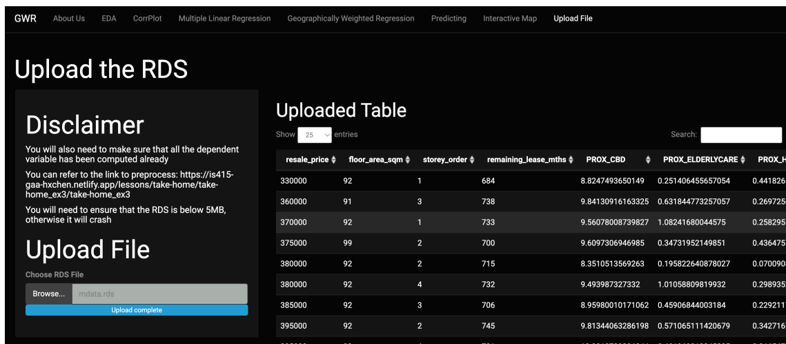
Fig. 8. Upload Tab
